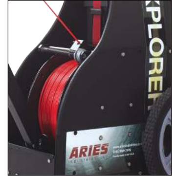
Automatic level wind enables faster, uniform camera retrieval
